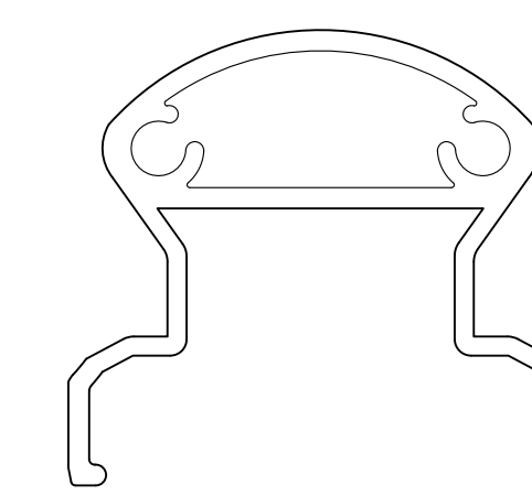
1520 INSIDE SLEEVE (sku# ZSL-05485-MIL)
