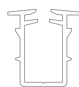
PVC INSERT FOR 5mm (sku# 23-26)
