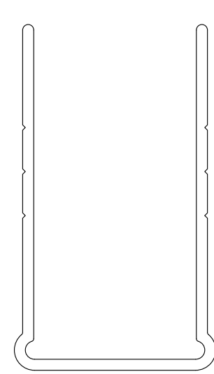
OPEN DEEP-H OUTSIDE SLEEVE (sku# SLV-02238-RAW)
