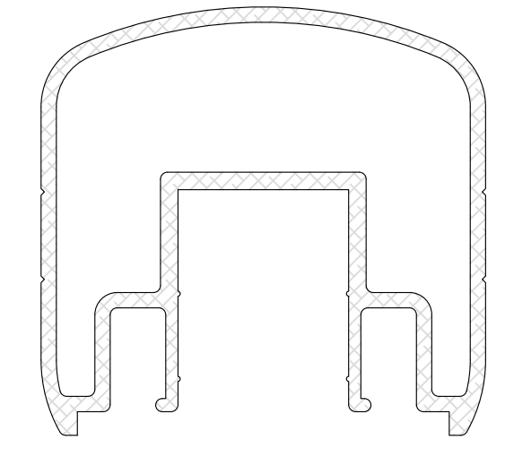
2000S SERIES (sku# 20-20)
