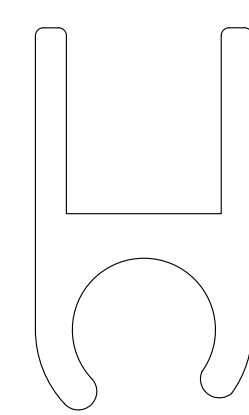
GLASS TRACK FOR CUSTOM ANGLE (sku# CHA-5000-RAW)
