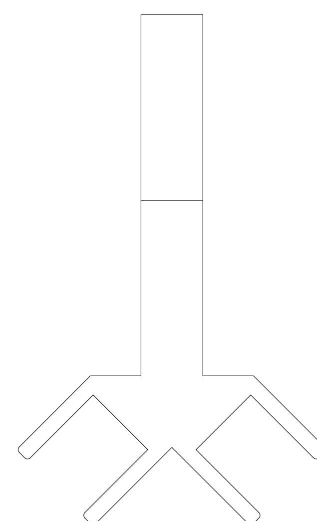
SIGNATURE POST MATERIAL-90° INSIDE (sku# PST-5030-RAW)
