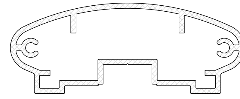
6100R TOP RAIL (sku# rai-01300-raw)
