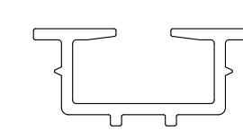
PVC CI-50 FOR 10/12mm (sku# 23-61)
