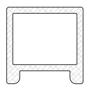
1100 SERIES CHANNEL (sku# RAI-01158-RAW)
