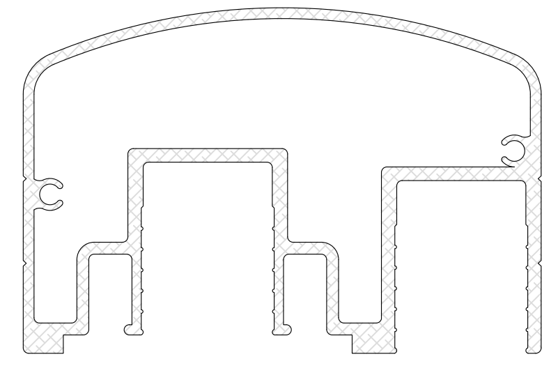
4000S TOP RAIL (sku# 04-20)
