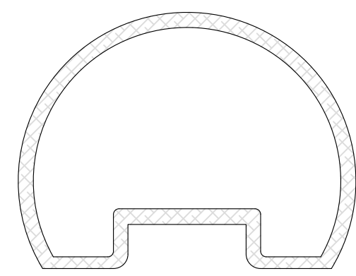
1900R TOP RAIL (sku# 10-30)
