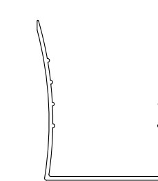
PVC CHANNEL FOR PICKET (sku# 25-05)
