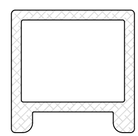
1100 SERIES CHANNEL (sku# RAI-01158-RAW)
