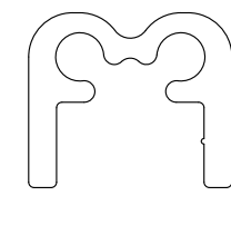
RAIL CLIP FOR DEEP-H (sku# 35-05)
