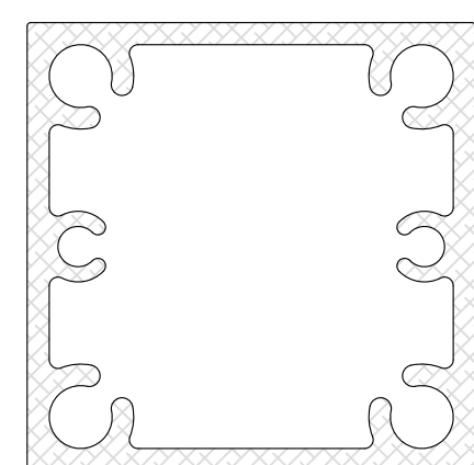
1-5/8" SQ. STANDARD POST (sku# 08-64)
