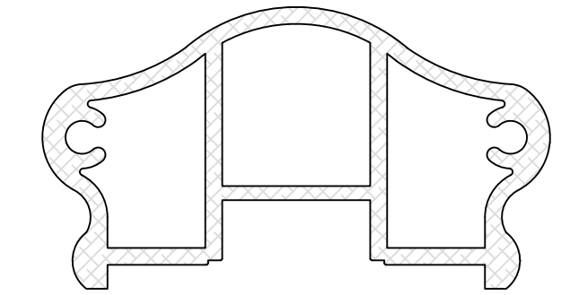
7000 TOP RAIL (sku# rai-01250-raw)
