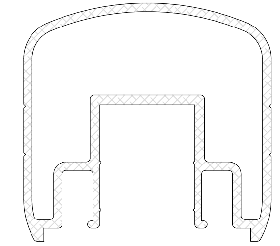
2000S SERIES (sku# 20-20)
