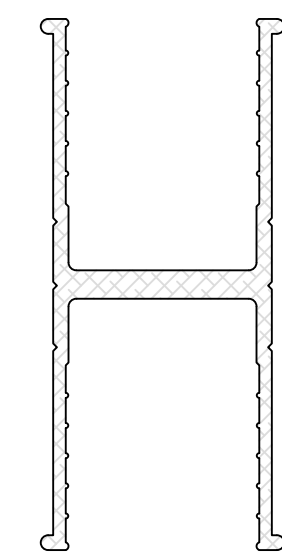
DEEP-H (DH) (sku# 25-02)
